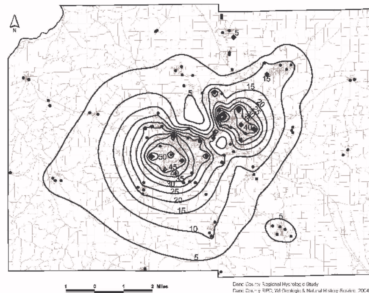
Figure 8. Simulated drawdown in Mt Simon aquifer, 1900-2000. Contours represent water level declines in feet.
