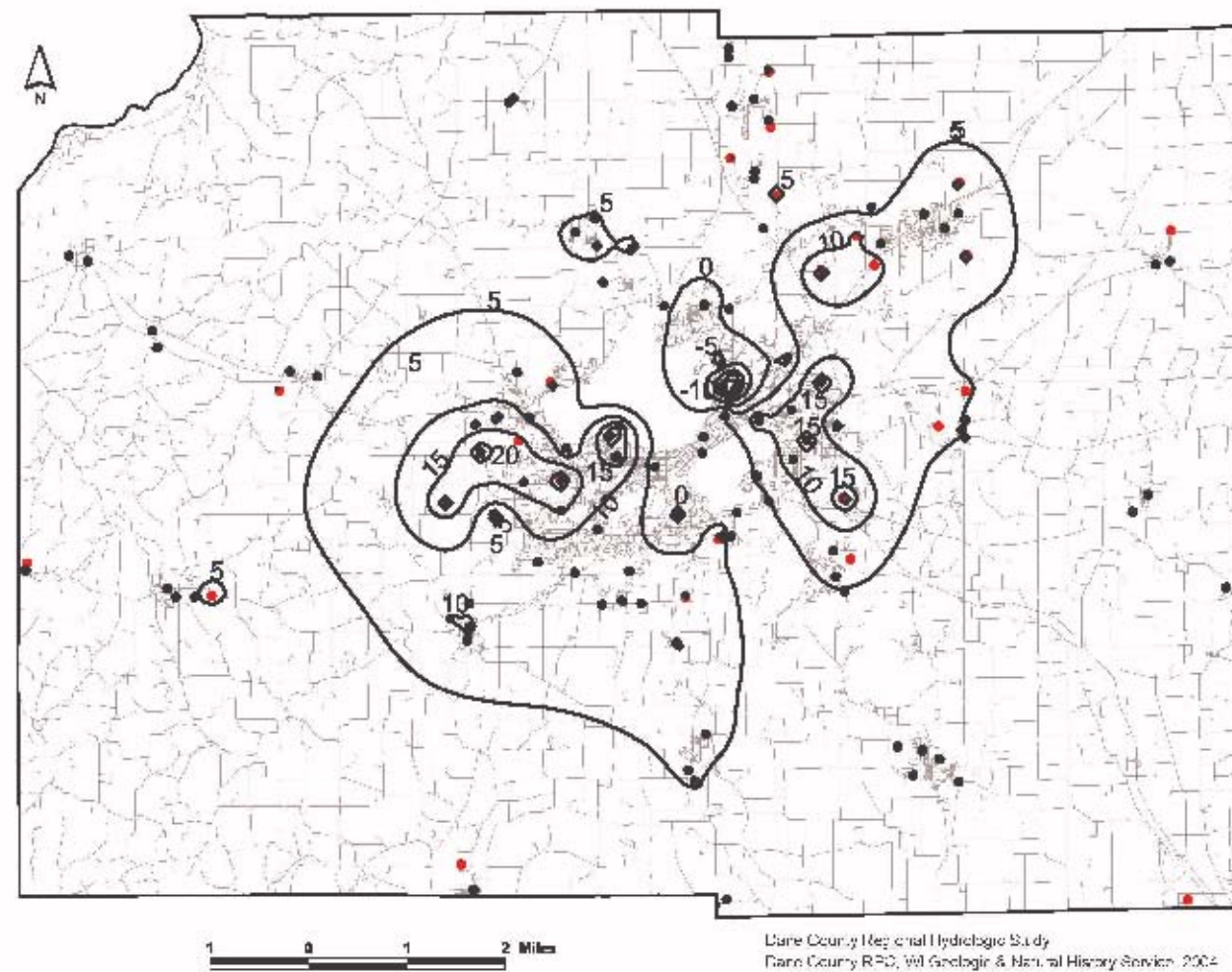
Figure 10. Simulated drawdown in Mt Simon aquifer, 2000-2030. Contours represent water-level declines in feet.
